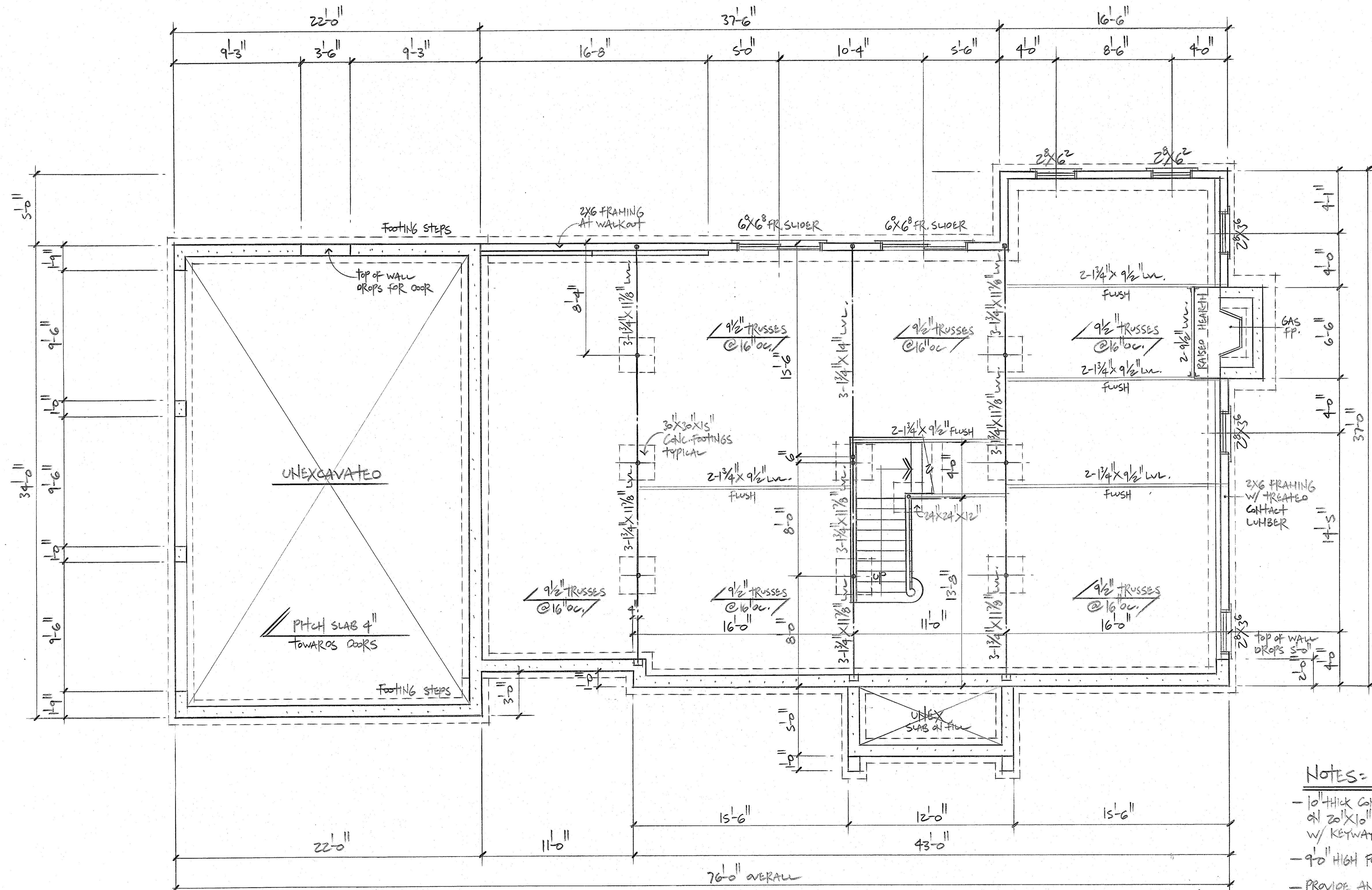
FOUNDATION PLAN
